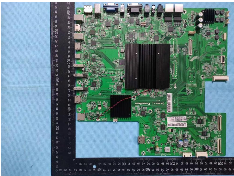
Figure 11. Interface board
