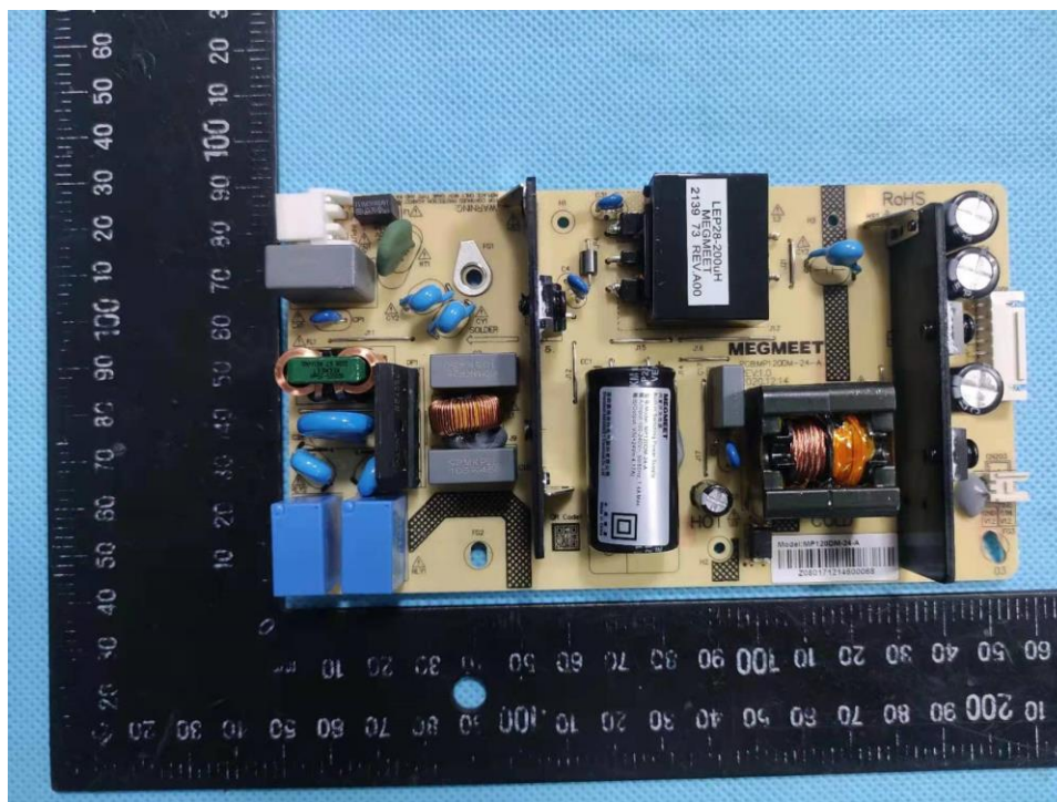
Figure 7. Power Board
