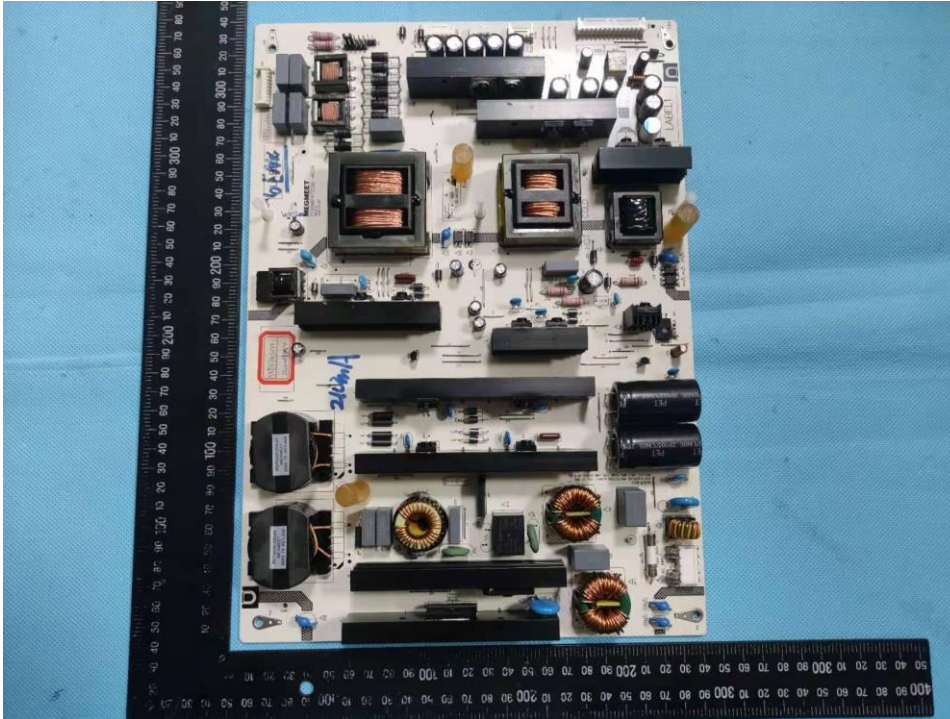
Figure 9. Power Board
