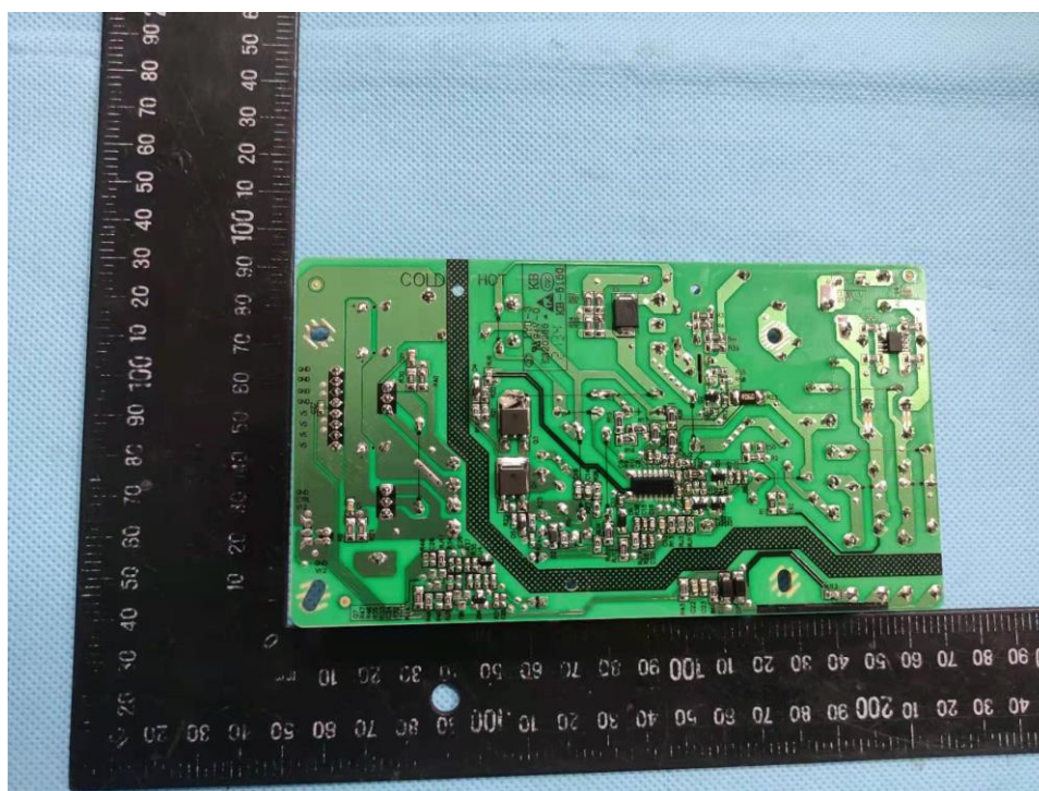
Figure 8. Power Board
