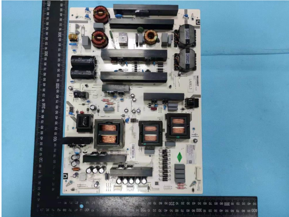
Figure 9. Power Board
